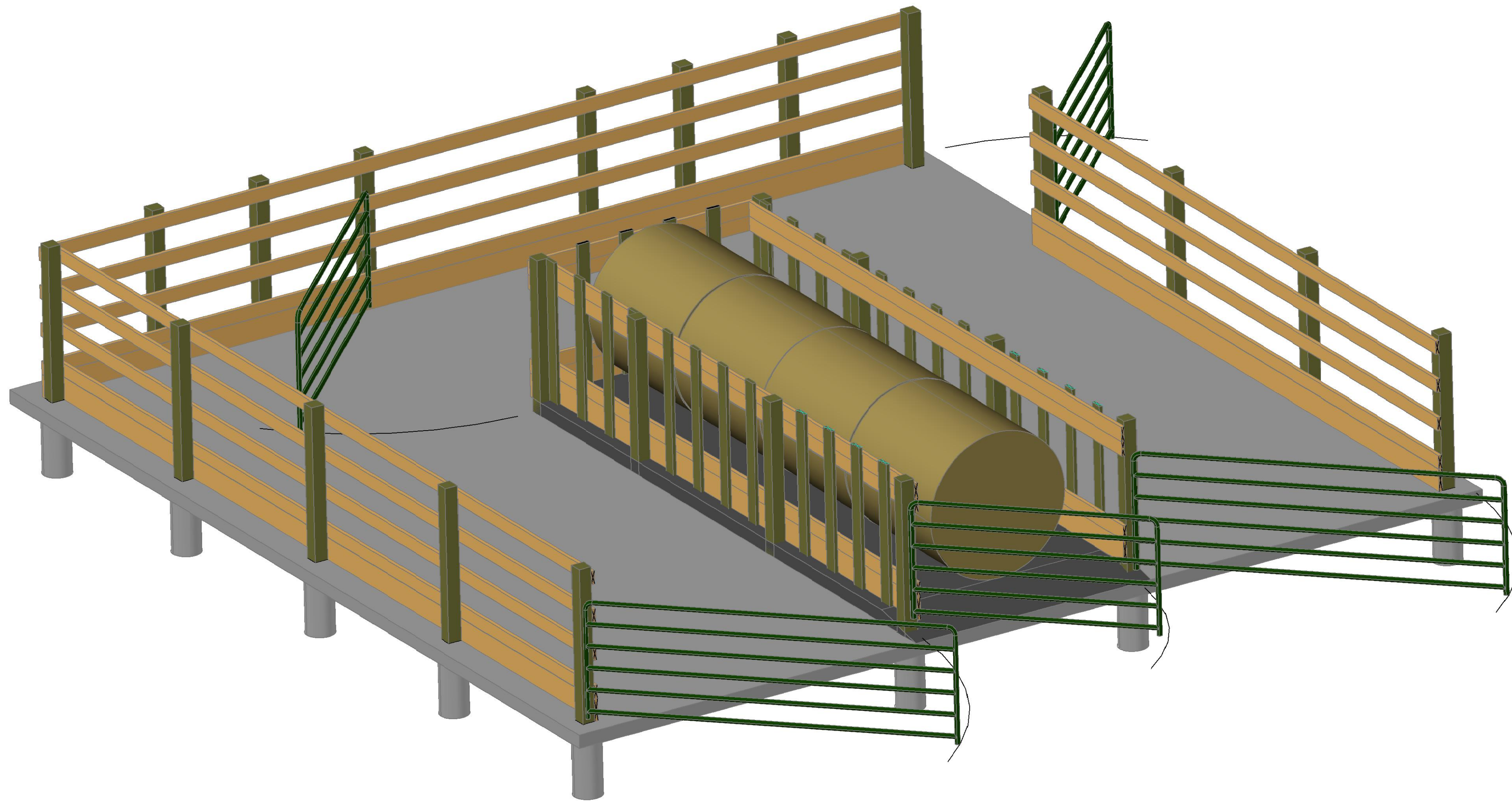
PERSPECTIVE VIEW
